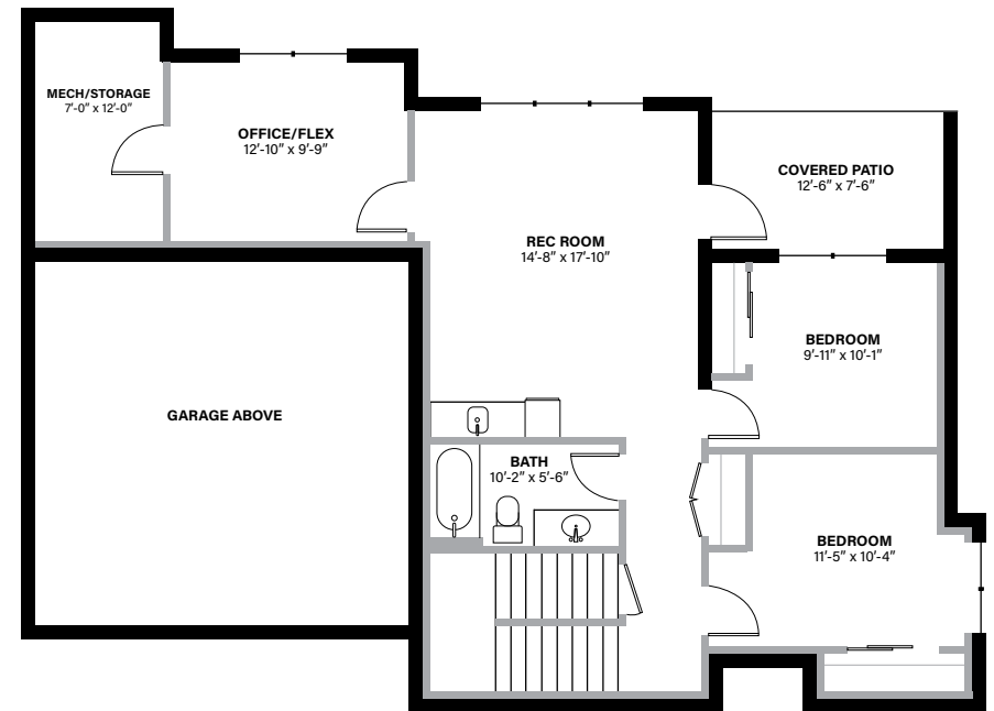
LOWER LEVEL
