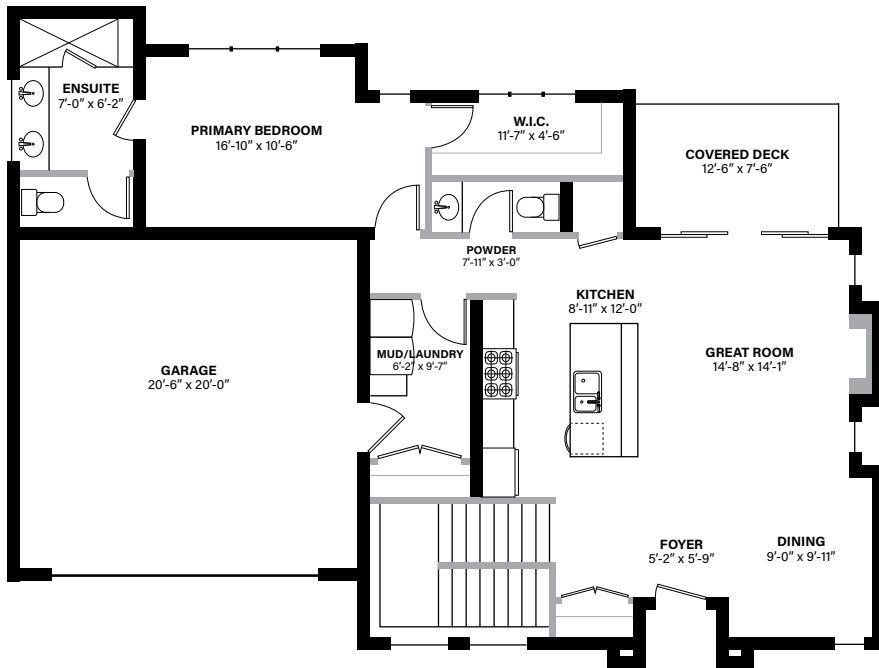
MAIN LEVEL
