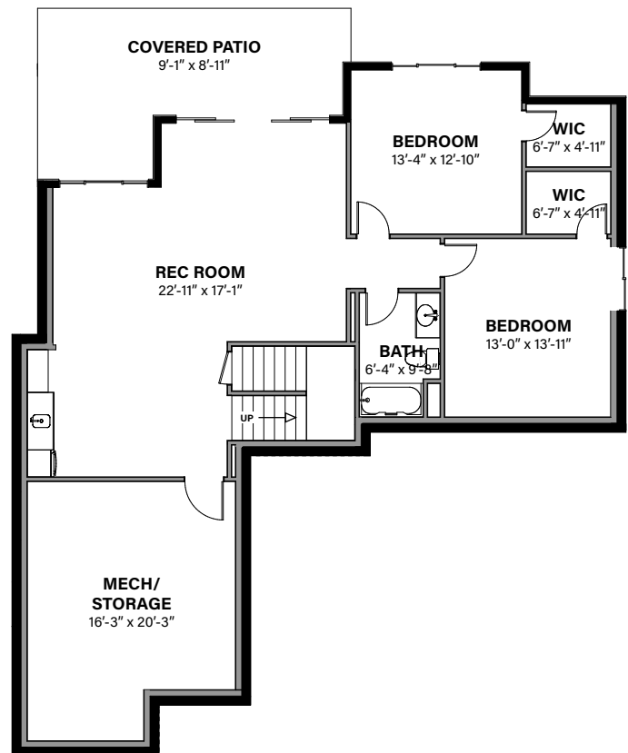
WALK-OUT LEVEL
