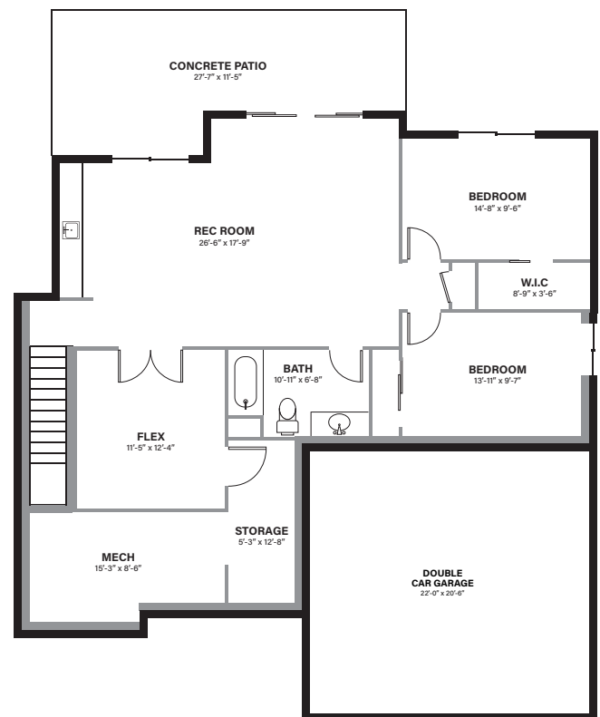
WALK-OUT LEVEL
