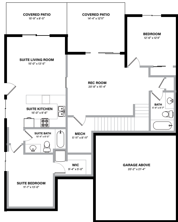
WALK-OUT LEVEL
