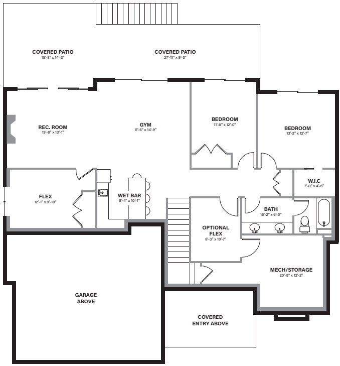
WALK-OUT LEVEL
