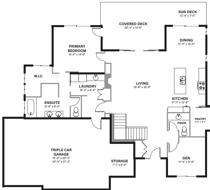
UPPER LEVEL
