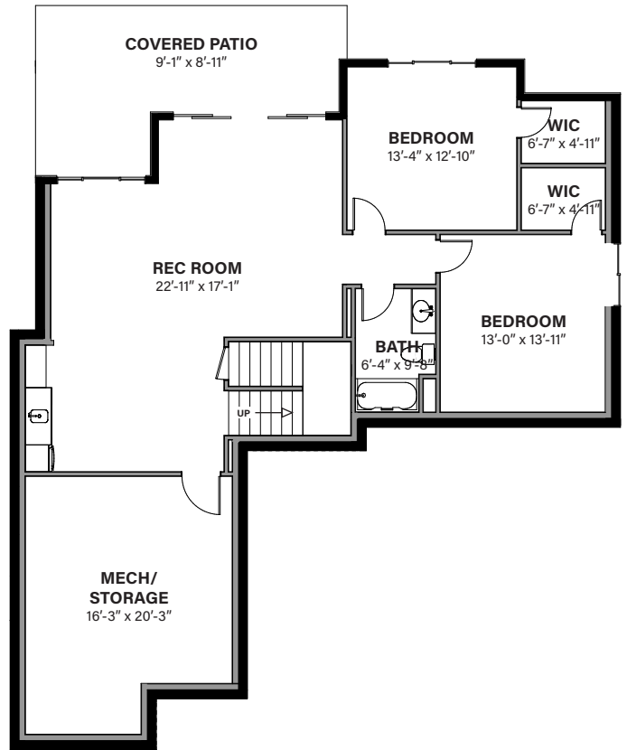
WALK-OUT LEVEL
