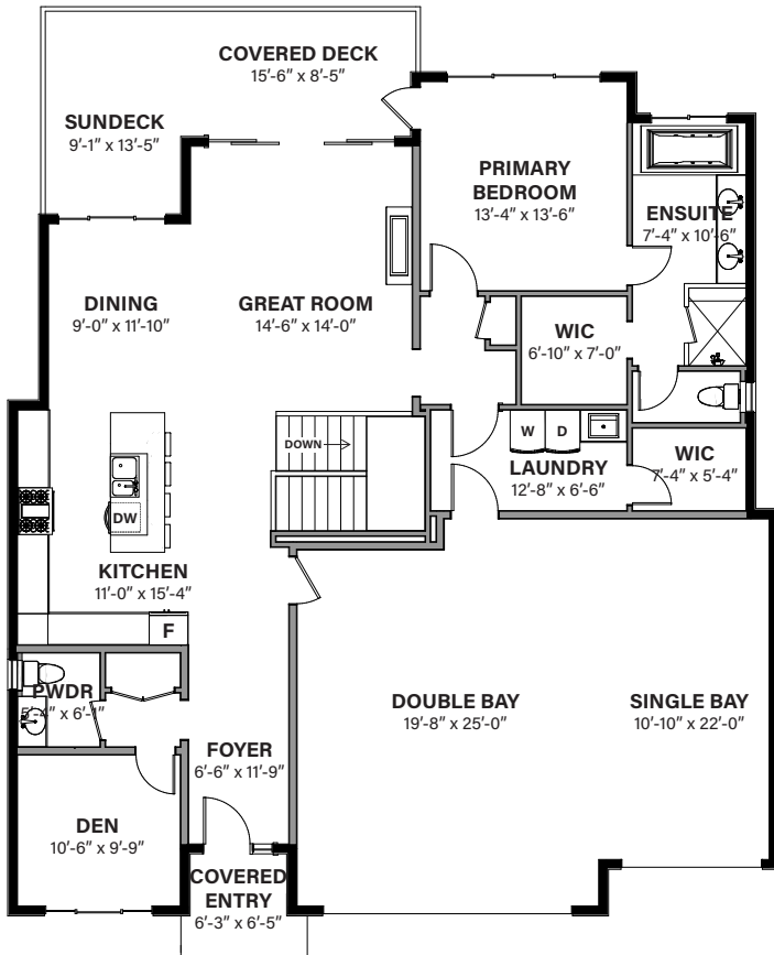
MAIN LEVEL
