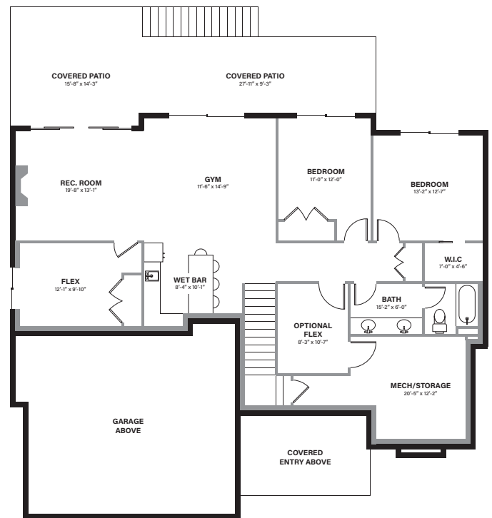
WALK-OUT LEVEL
